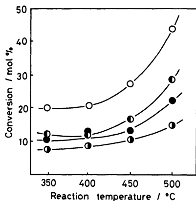
Fig. 1. Effect of reaction temperature on conversion of OCT. HM catalyst having \text{SiO}_2/\text{Al}_2\text{O}_3 mol ratio of 19.0 was used as a catalyst after treatment with \text{CF}_3\text{Cl} ; the treatment was carried out at 450^\circ\text{C} for 8 min. W/F=64.9 gh/mol. Symbols used in this figure are as following.
